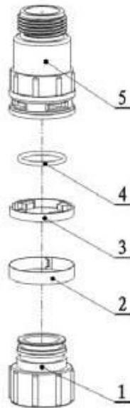
5457002 Animated Connector
