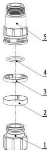
5457002 Animated Connector
