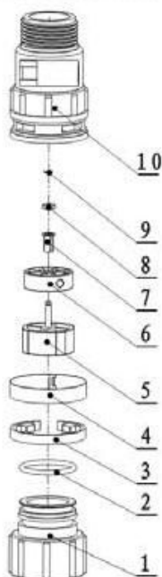
5447001 Flow Meter
