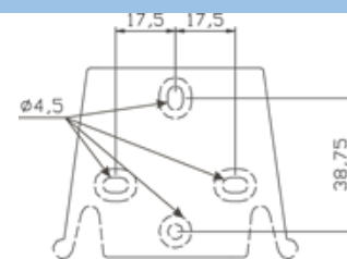
WALL bracket
